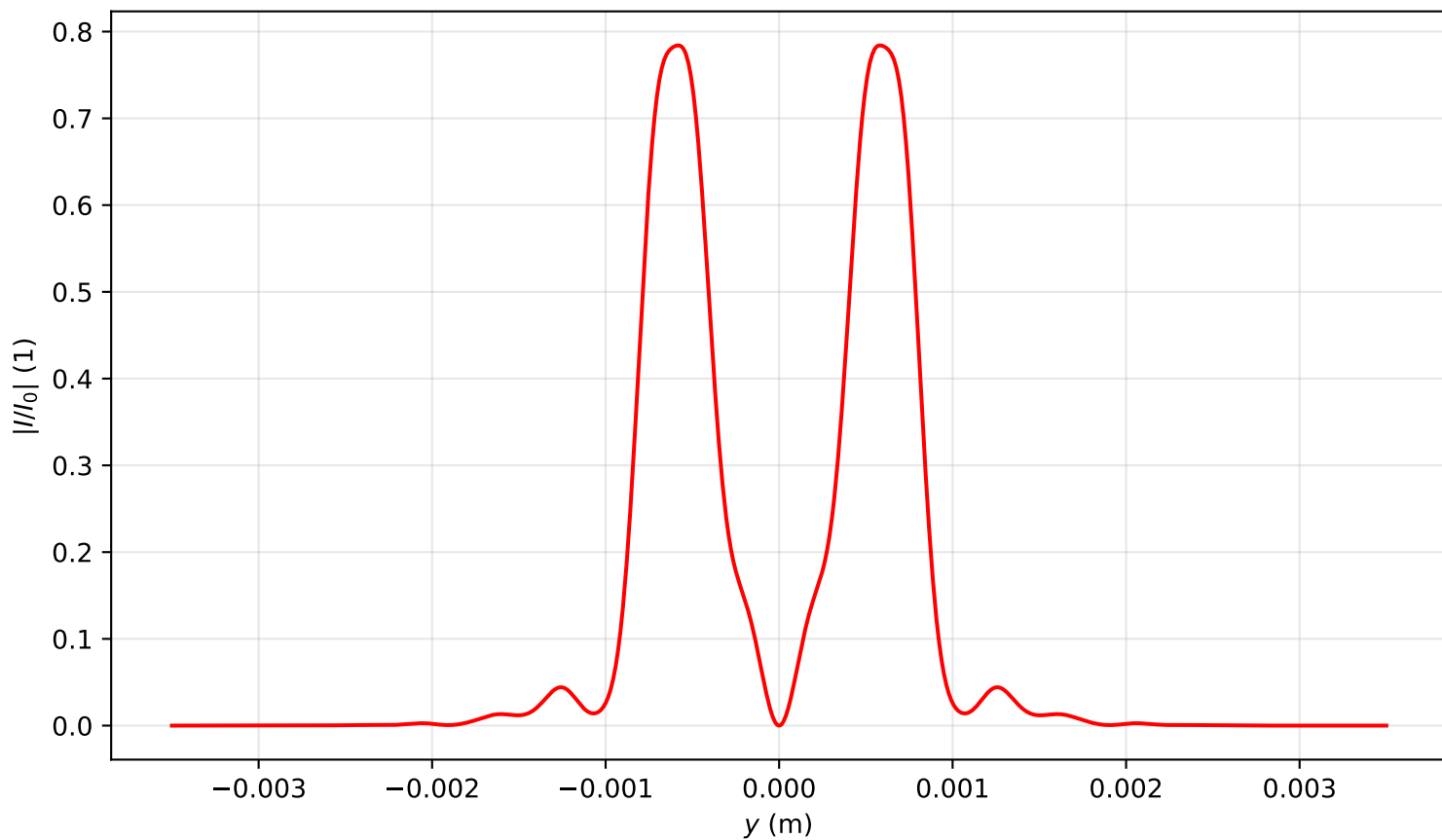
Intensity profile I(x=0, y, z=1.274)/I_0 , P_{in}=7.0P_{cr} , artificial time
